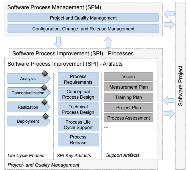
Figure 1: The ArSPI model (overview).
